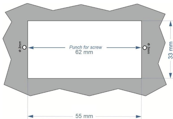
Door cut out
